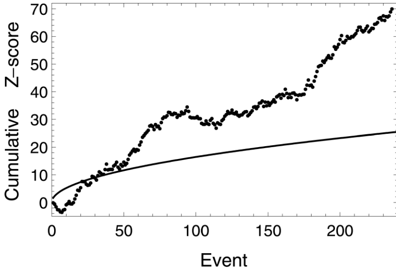
Fig. 3. The summed chronological deviation of 236 event z-scores. Each point represents the contribution from the normal z-score of a single event. The null expectation is zero and the parabola gives a 5% probability envelope for positive deviation. The relatively steady trend shows that the cumulative deviation is broadly distributed among many events and is not due to outlier events.
